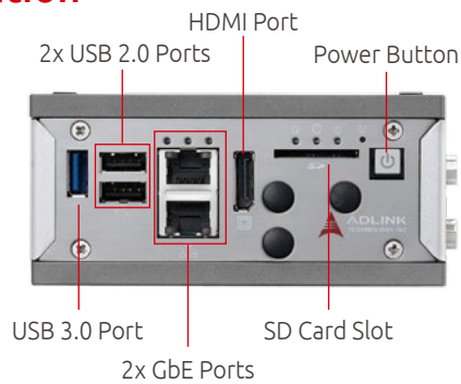
Front view of MXE-200/200i
