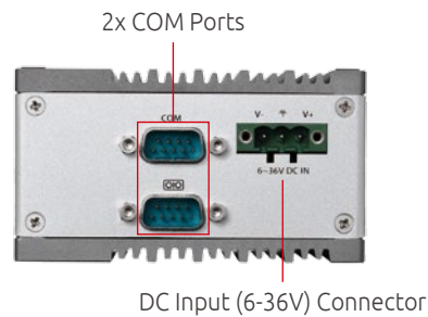
Right side view of MXE-200/200i
